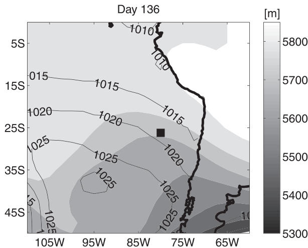
FIG. 18. As in Fig. 11 but for day 136.
