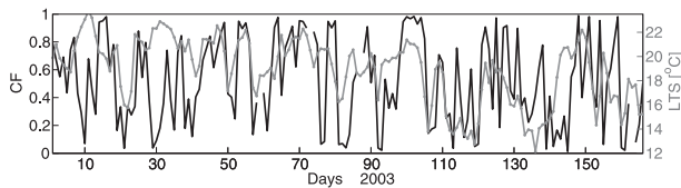
FIG. 4. Time series for the daily mean CF (black line) and daily mean LTS (gray line). For the mean CF, we excluded the hours 1–5 LST (period of power restriction; see the text for more information).
