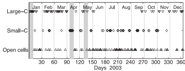
FIG. 7. Time series for the occurrence of closed and open cells over SFI during 2003. Gray bars indicate the time periods corresponding to the examples shown in Figs. 11, 14, and 17.
