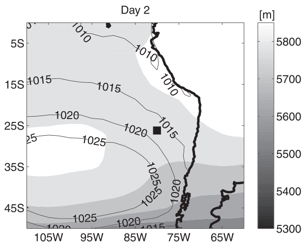
FIG. 12. SLP (contours) and geopotential height at 500 hPa (shaded) for day 2.
