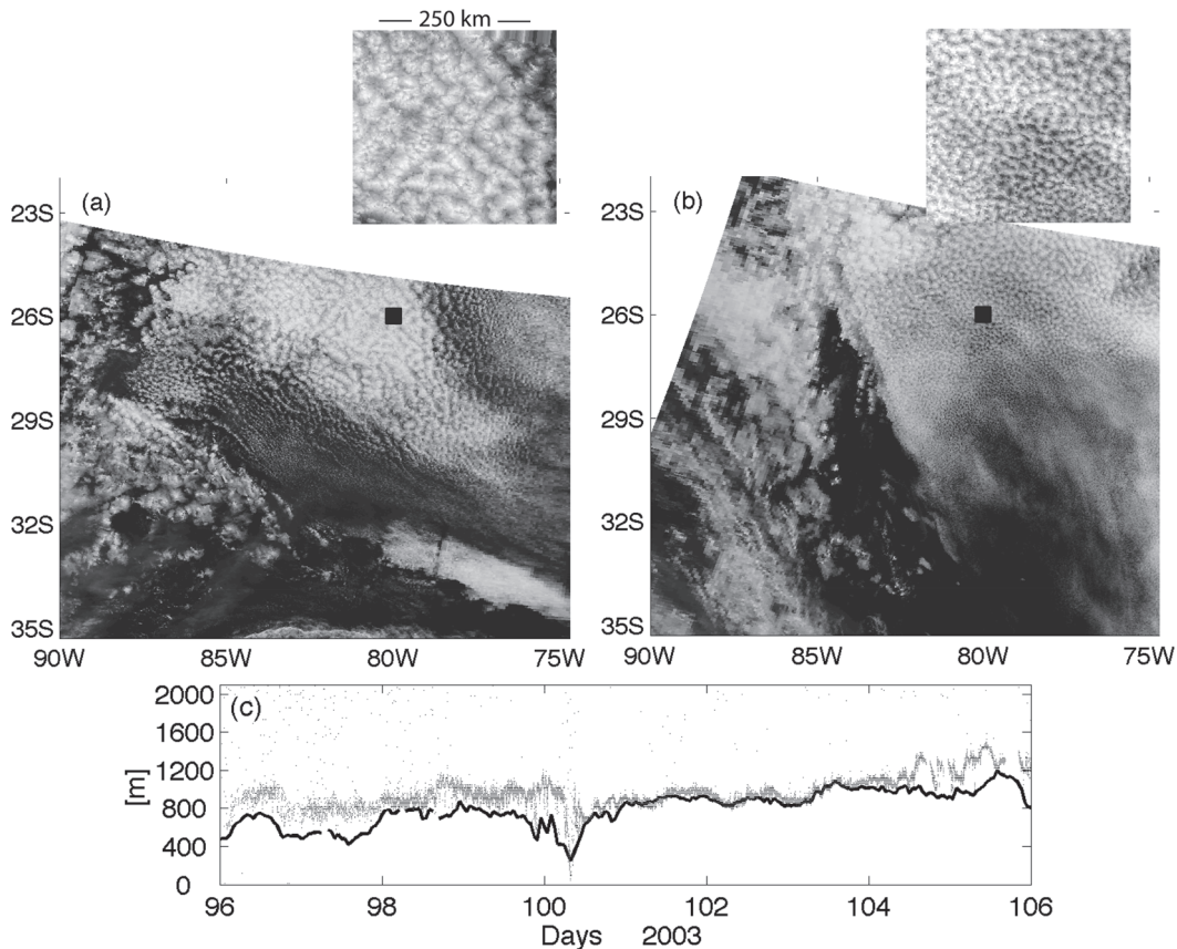
FIG. 14. As in Fig. 11 but for a small closed-cell period: (a) day 98 (8 Apr), (b) day 102, and (c) ceilometer cloud bases and LCL (black line).
