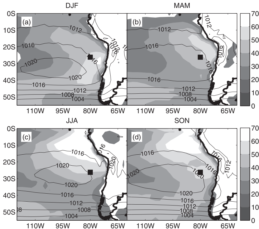
FIG. 1. Seasonal means in warm-cloud cover (shaded) derived from ISCCP (1983–2007; D2 data; Rossow and D  nas 2004) and corresponding NCEP–NCAR reanalysis (Kalnay et al. 1996) sea level pressure means (contours) for austral (a) summer (December–February), (b) autumn (March–May), (c) winter (JJA), and (d) spring (SON). The location of SFI is represented by the dark square.
