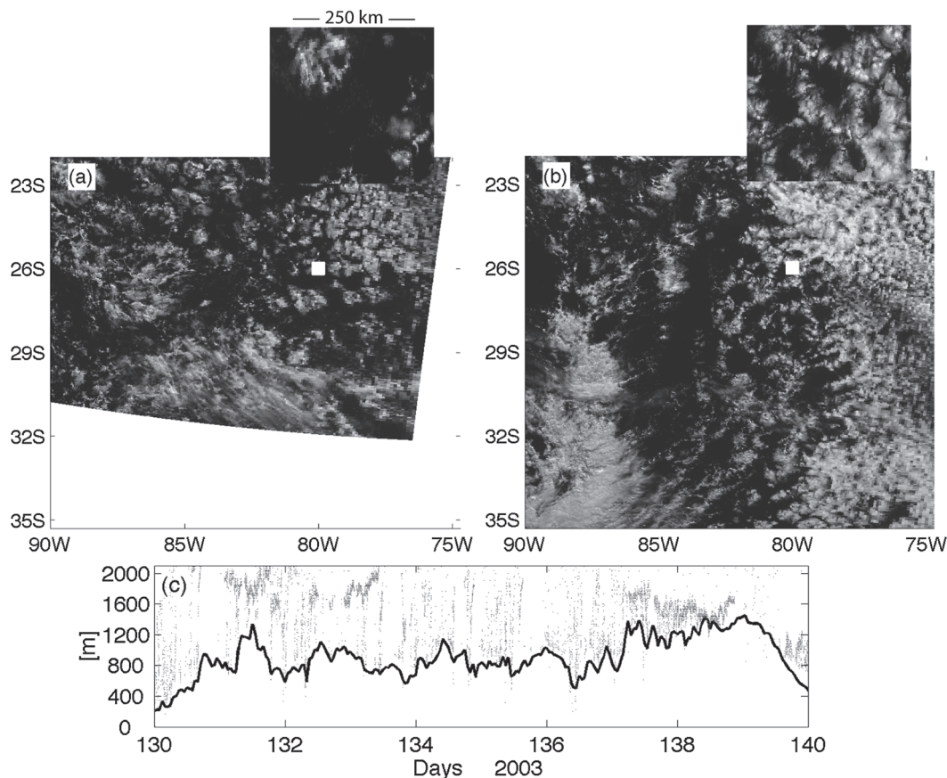
FIG. 17. As in Fig. 11 but for an open-cell-like period: (a) day 135 (15 May), (b) day 137, and (c) ceilometer cloud bases and LCL (black line).
