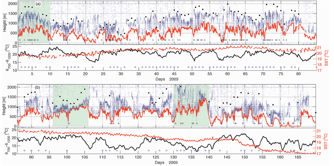
FIG. 3. Time series for CBH (blue dots, each 30 s), LCL (red line), and daily-mean CTH (black circles). Human-detected drizzle and AWS-reported light rain are represented by open circles and crosses, respectively. In the bottom plot of each panel, the black line corresponds to LTS, the red line to SST, and blue open circles to the Cu-under-Sc reports. The time series starts on 1 Jan, showing (a) JFM and (b) AMJ. Horizontal ticks below the 0 level indicate periods with no ceilometer records.
