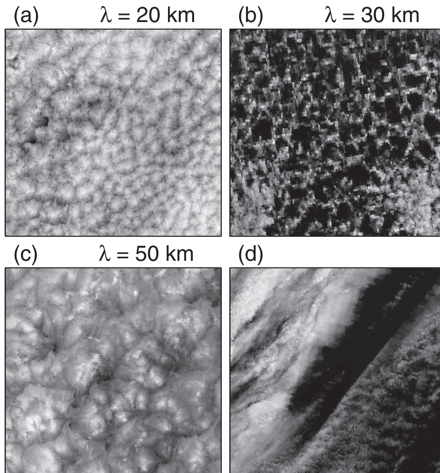
FIG. 2. Three cellular patterns: (a) small closed cells (28 Apr), (b) open cells (7 Jul), and (c) large closed cells (10 Jan), and (d) an example without cellular structure (18 Aug). The images of the cellular structure centered at SFI are 250 \text{ km} \times 250 \text{ km} . Typical wavelengths ( \lambda ) are indicated on the right upper corner of each image.
