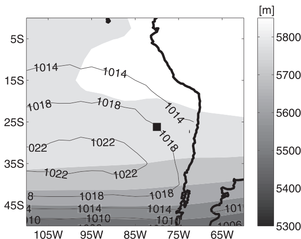
FIG. 10. Large closed cell composite. Contours indicate SLP and shading geopotential height at 500 hPa. The thick square represents the location of SFI.
