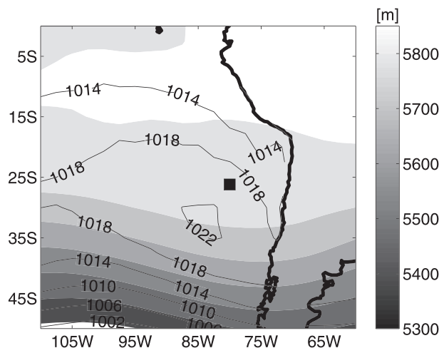
FIG. 13. Small closed-cell composite. Contours indicate SLP and shading geopotential height at 500 hPa. The thick square represents the location of SFI.
