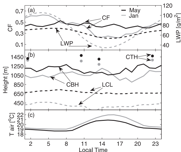
FIG. 6. Mean diurnal cycles for January (gray) and May (black) 2003 of ceilometer-derived (a) low CF and LWP (dashed line). (b) CBH (solid line), LCL (dashed lines), and CTH (dots; gray line is the diurnal cycle for January–February and the black line for May–June). (c) Diurnal cycle of the island temperature recorded by AWS.
