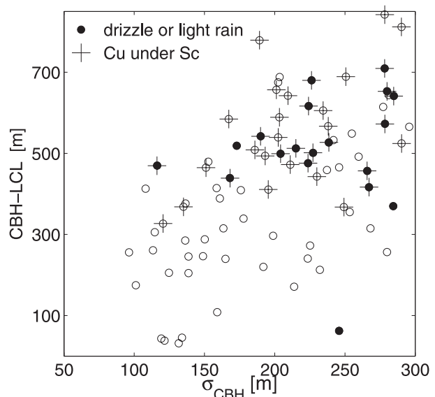
FIG. 5. Scatterplot between the daily standard deviation of CBH ( \sigma_{CBH} ) and CBH–LCL. The black circles indicate events with drizzle or light rain and the crosses represent days with presence of Cu-under-Sc. They are only considered events when there are at least two daily reports of drizzle or Cu-under-Sc.
