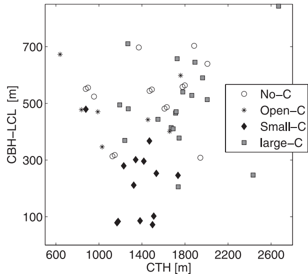
FIG. 8. Scatterplot between daily CTH and CBH-LCL. The small closed and large closed cells are represented by black diamonds and gray squares, respectively, whereas the open cells are represented by asterisks. Open circles indicate no-cellular structures. Only overcast pixels were used.
