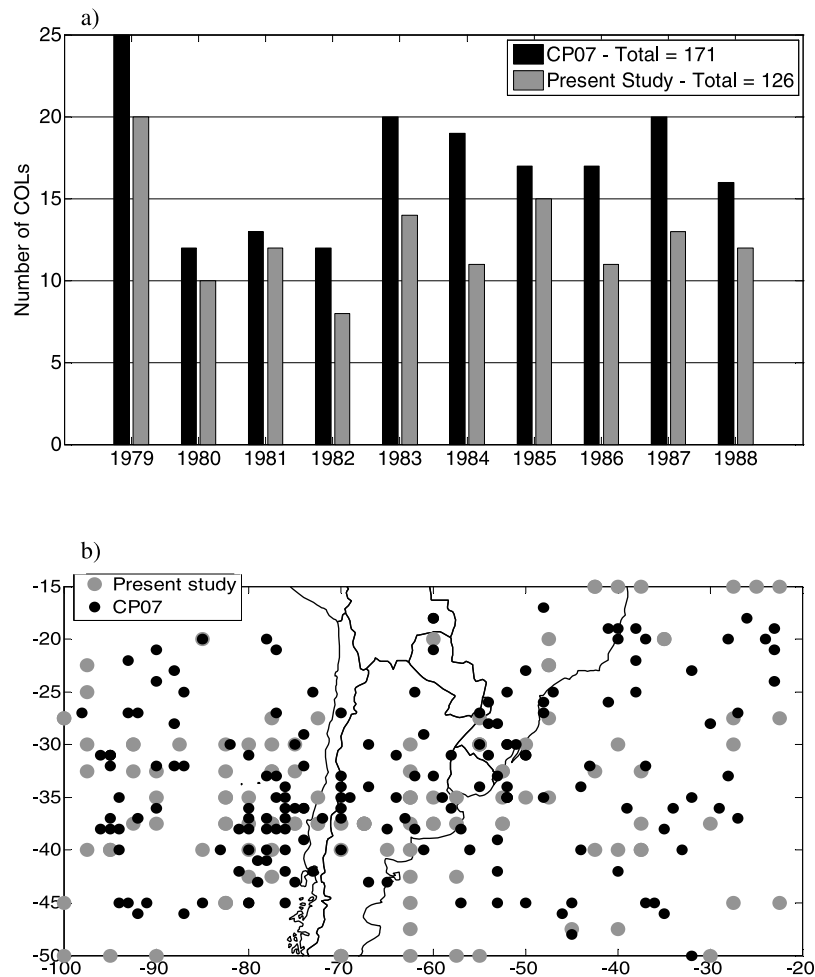
Figure 2. (a) The annual number of COLs at 250 hPa in CP07 (black bars) and at 200 hPa in the present study (gray bars) and (b) the spatial distribution of COLs from 1979 to 1988 in the region between 15°S–50°S and 100°W–20°W. In Figure 2b, gray circles indicate the first position of COLs detected by the method used in this study, and black circles represent the greatest depth of COLs detected by CP07.
