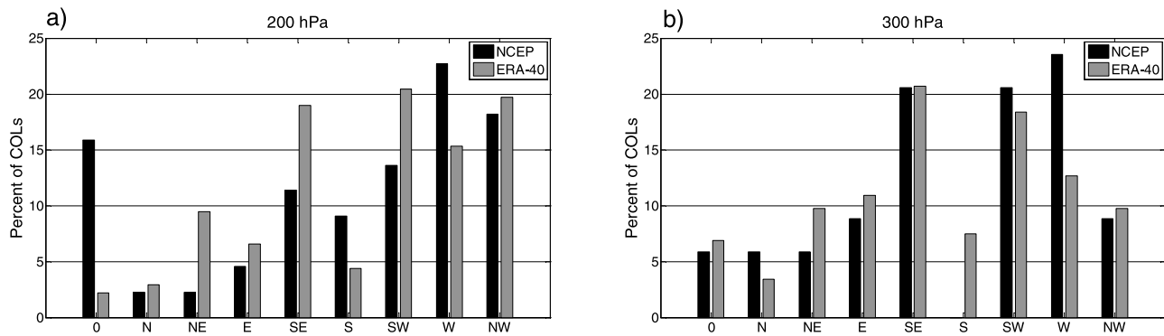
Figure 11. Similar to Figure 10, but for the displacement of COLs over the northeast of Brazil ( 10^{\circ}\text{S} – 25^{\circ}\text{S} , 20^{\circ}\text{W} – 55^{\circ}\text{W} ).
