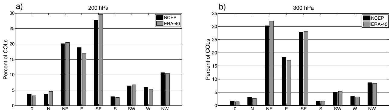
Figure 10. The direction of displacement of the COLs in the SH from 1979 to 1999 in the NCEP-NCAR and ERA-40 at (a) 200 hPa and (b) 300 hPa. The horizontal axis shows the direction of movement directions; stationary COLs are represented by 0.
