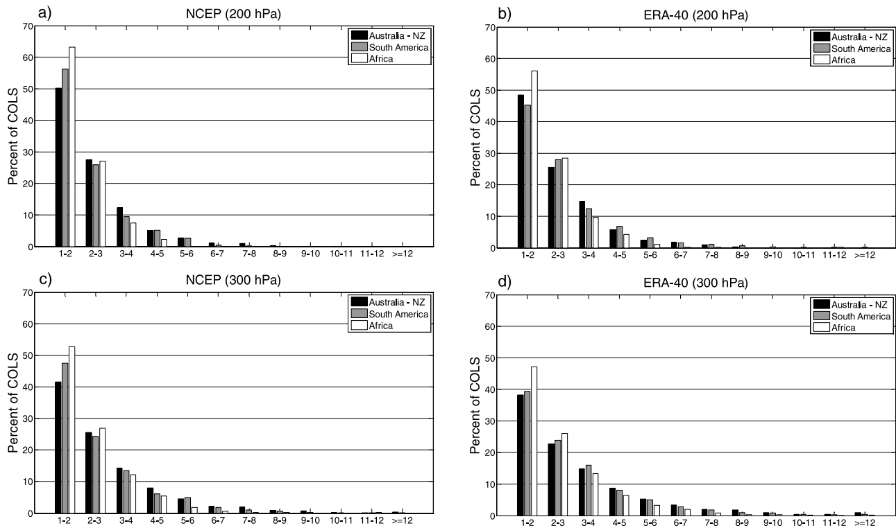
Figure 6. The frequency distribution with respect to the lifetime of COLs, in days, for the Australia–New Zealand (60°E–130°W), South America (130°W–20°W), and southern Africa (20°W–60°E). The frequency intervals do not include the last number.
