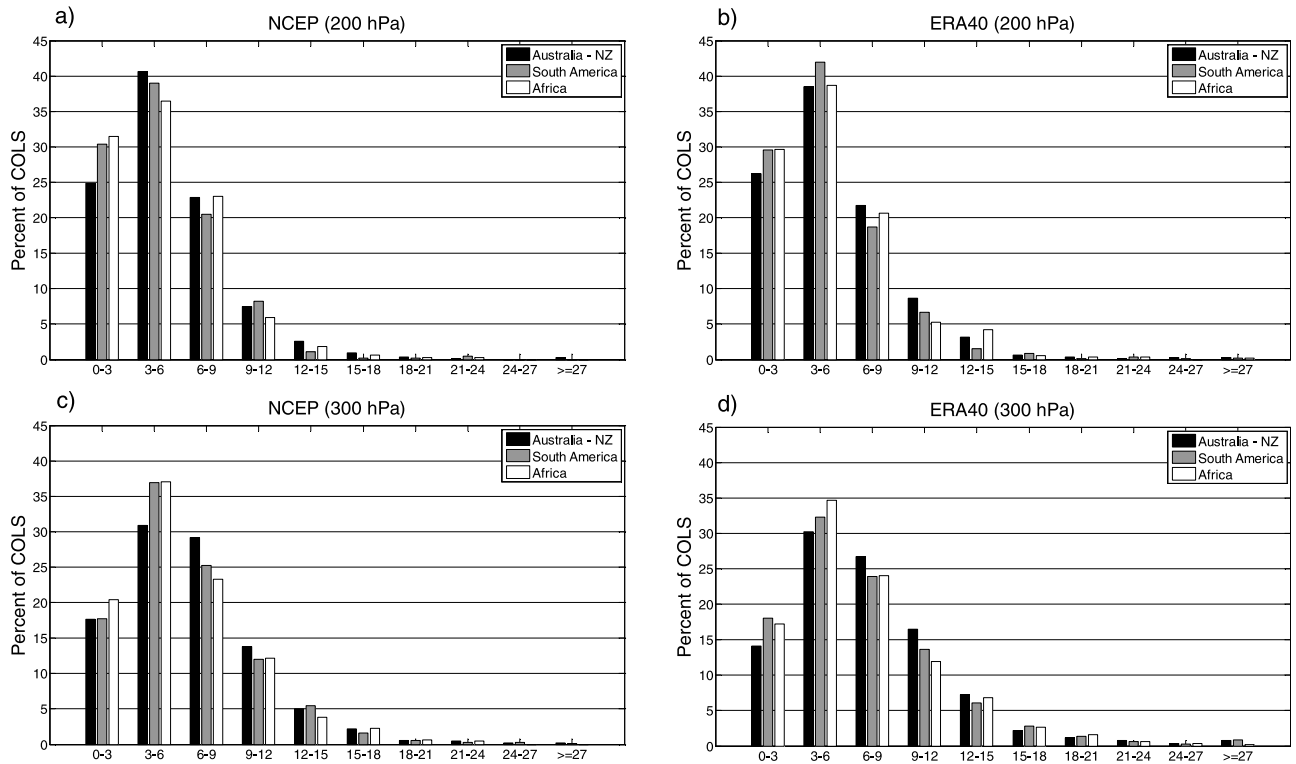
Figure 7. As in Figure 6, but for the mean velocity of COLS (m s -1 ).
