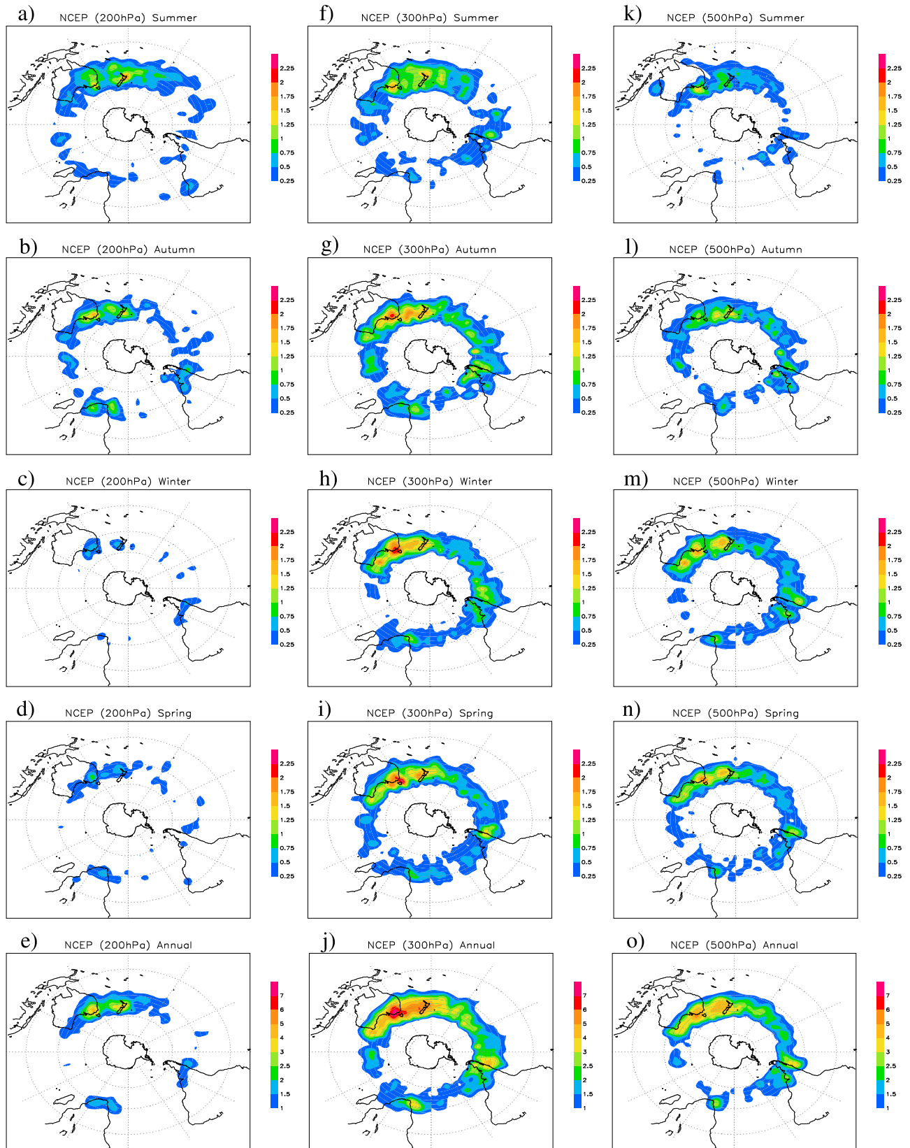
Figure 4. The seasonal and annual average density ( \times 10^5 \text{ km}^{-2} ) of the occurrence of COLs in their initial position in the NCEP-NCAR reanalysis at (a–e) 200 hPa, (f–j) 300 hPa, and (k–o) 500 hPa. The density corresponds to the number of COLs in squares of 2.5^\circ latitude \times 2.5^\circ longitude, normalized by their areas, divided by the number of seasons and smoothed twice with a 9 \times 9 point moving average.
