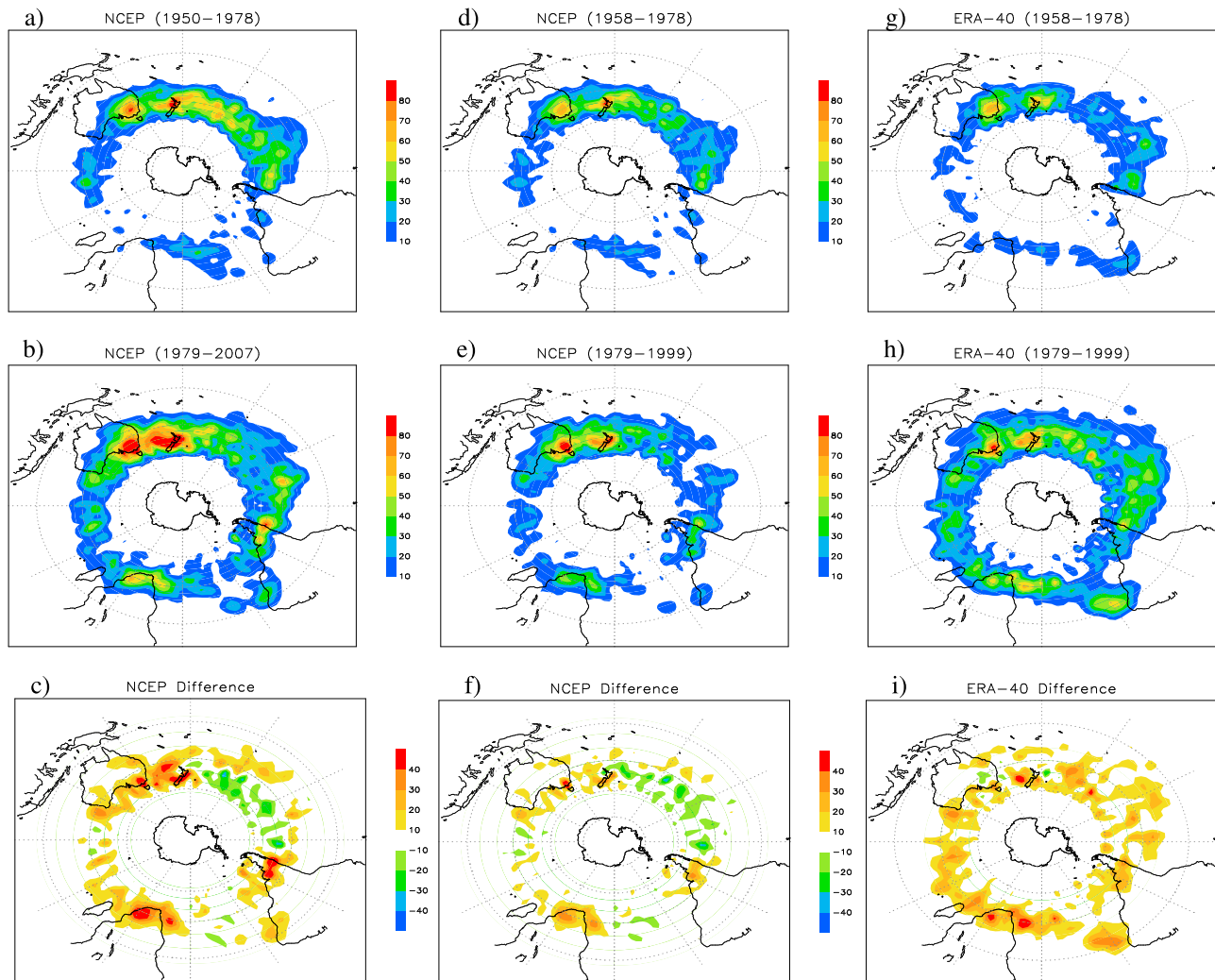
Figure 3. The total density ( \times 10^5 \text{ km}^{-2} ) of the occurrence of COLs in their initial position at 200 hPa in the (left and middle) NCEP-NCAR and (right) ERA-40 reanalyses for pre- and post-1979. (a) From 1950 to 1978, (b) from 1979 to 2007, and (c) the difference between Figures 3a and 3b in the NCEP-NCAR. (d) From 1958 to 1978, (e) from 1979 to 1999, and (f) the difference between Figures 3d and 3e in the NCEP-NCAR. (g) From 1958 to 1978, (h) from 1979 to 1999 and (i) the difference between Figures 3g and 3h in the ERA-40. The density corresponds to the number of COLs in squares of 2.5^\circ latitude \times 2.5^\circ longitude normalized by their areas and smoothed with a 9 \times 9 point moving average.
