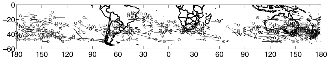
Figure 9. The trajectories of COLs at 200 hPa in the NCEP-NCAR reanalysis during 1979, 1980, 1981, 1990, and 1993 (neutral years, without El Niño or La Niña events). Circles indicate the final position of the COLs.
