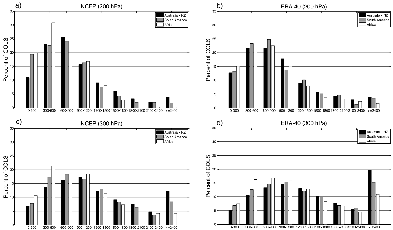
Figure 8. As in Figure 6, but for the distance traveled by the COLS (in km).
