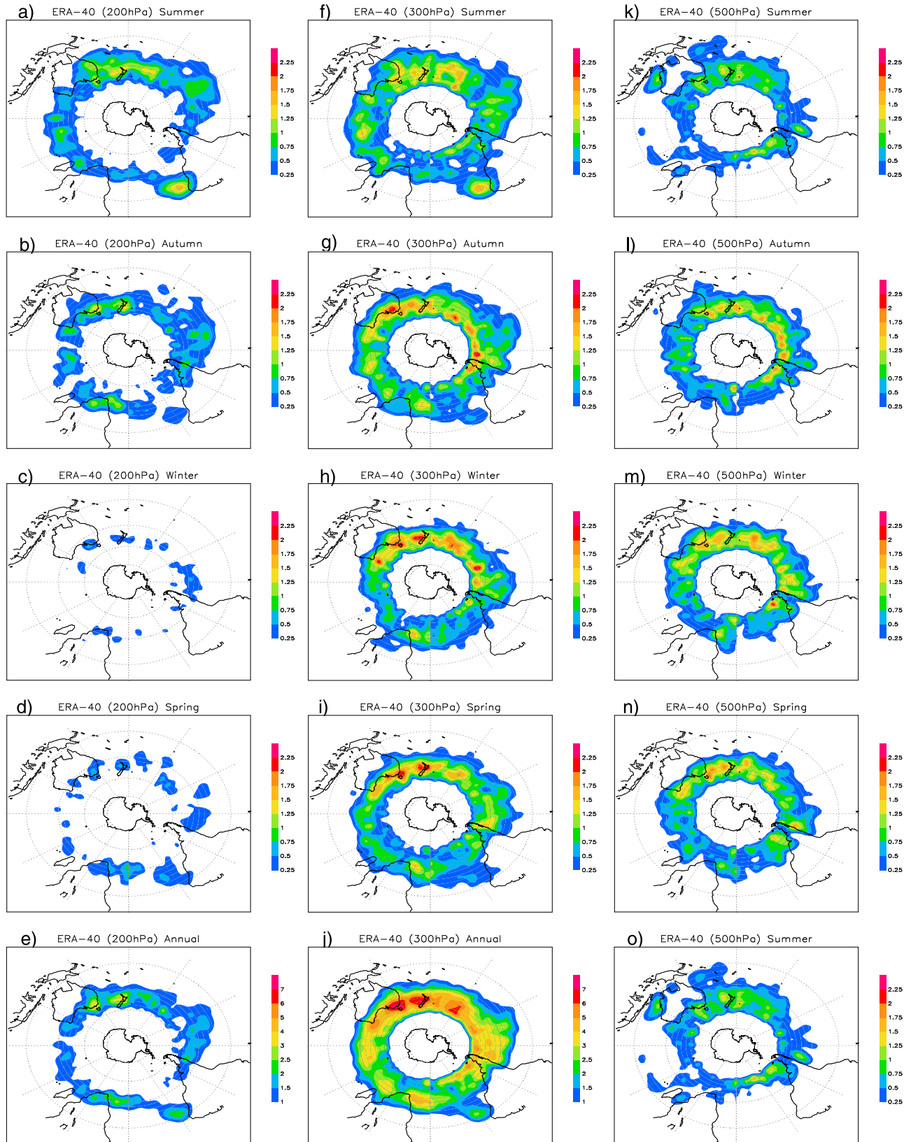
Figure 5. As in Figure 4, but for the ERA-40 reanalysis.
